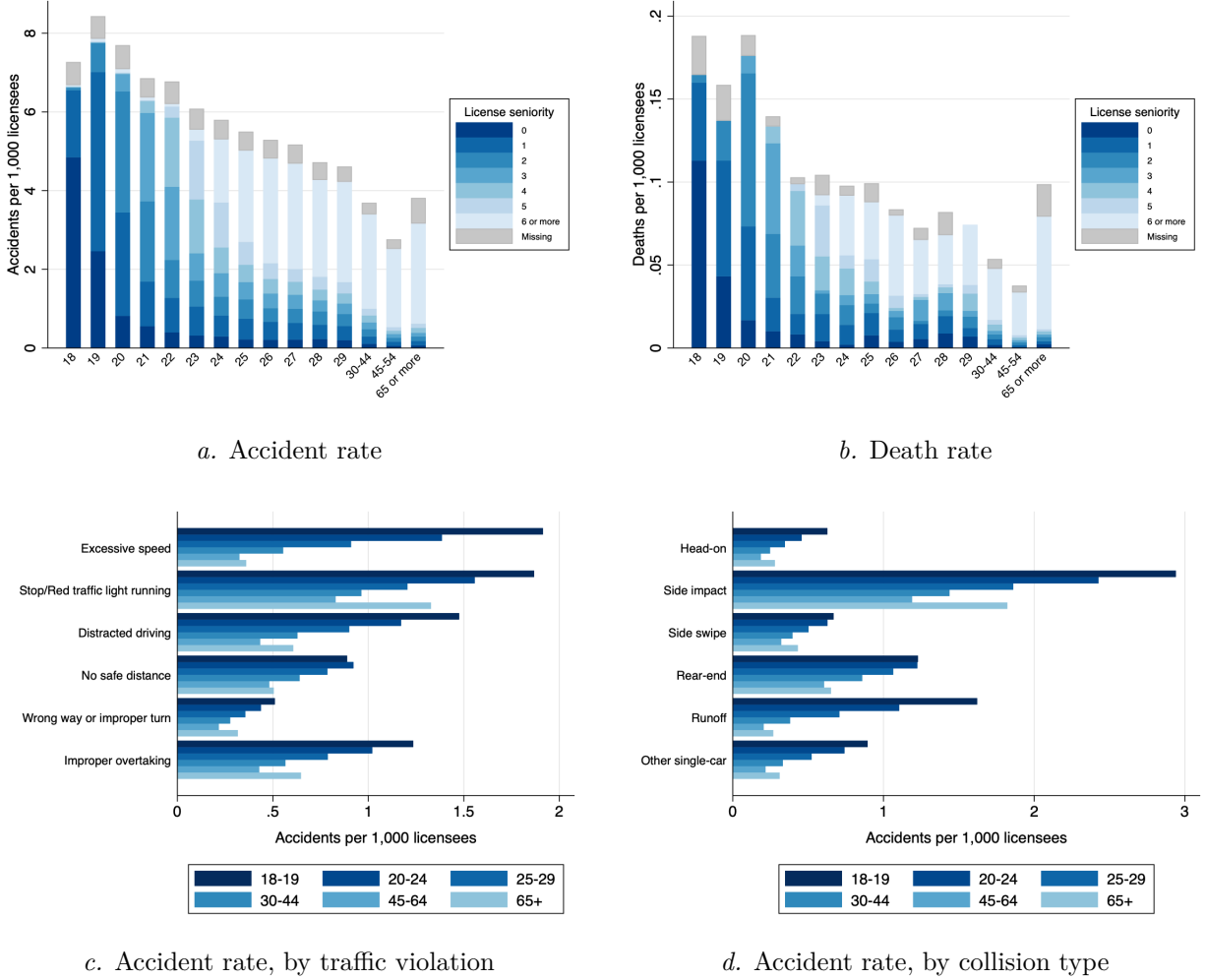
Figure I: Summary Statistics
