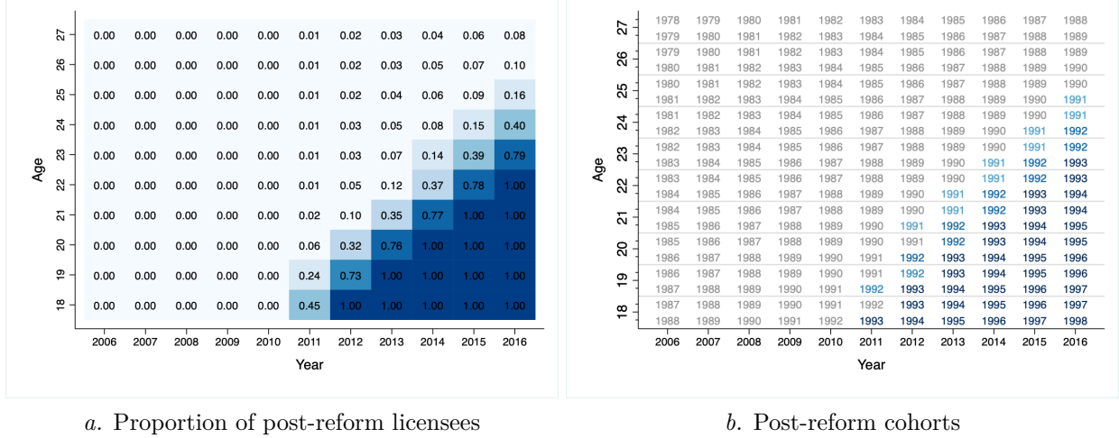
Figure III: Post-reform Licensees
