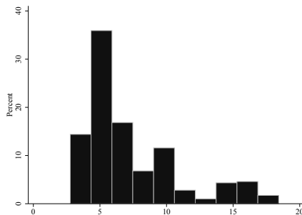
Figure B.1: Distribution of \sigma_b , 2008-2013
