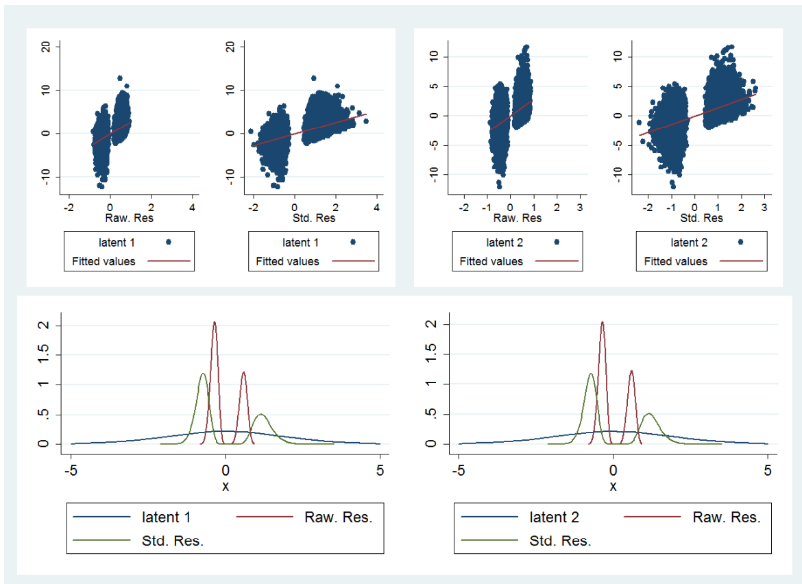
Figure 3: True latent factors against estimated residuals
