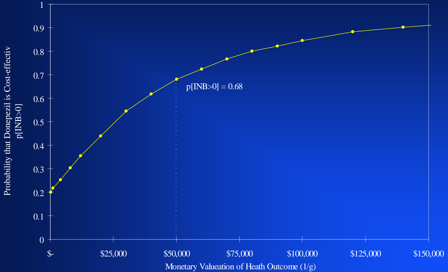
Figure 2b Acceptability curve for Donepezil
