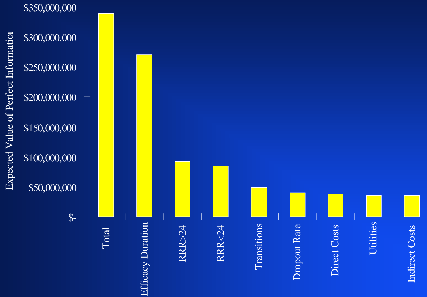
Figure 4 EVPI for model inputs (210 weeks)
