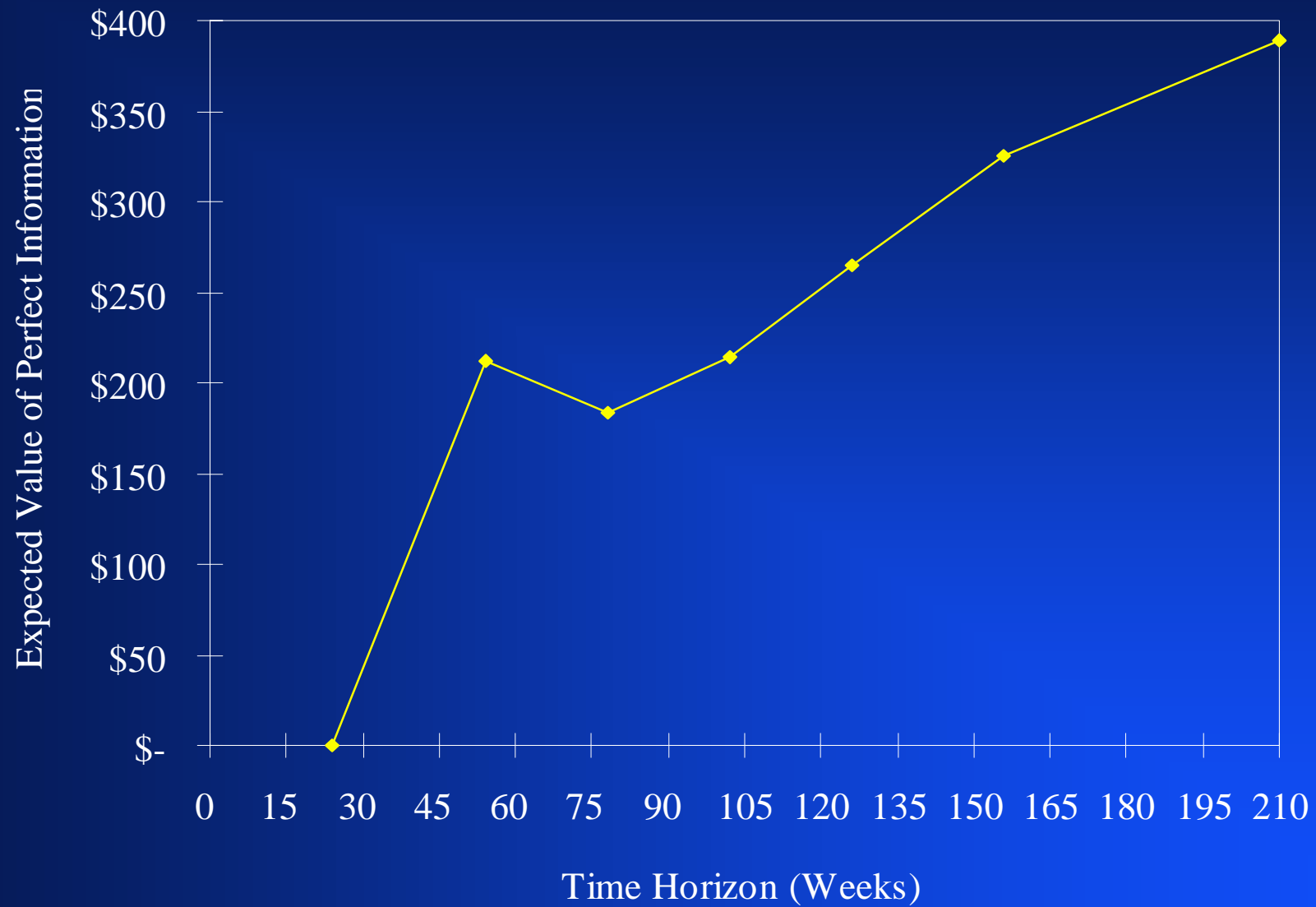
Figure 3a EVPI for an individual patient
