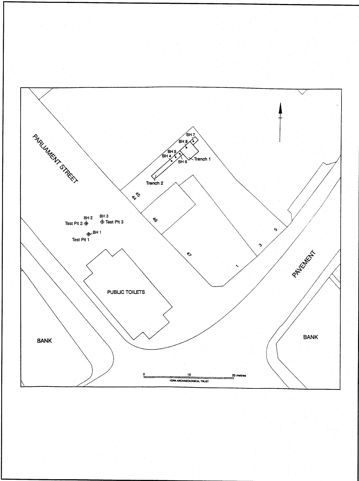
Figure 3. 44-5 Parliament Street, York: site plan showing trenches within building and locations of boreholes.
