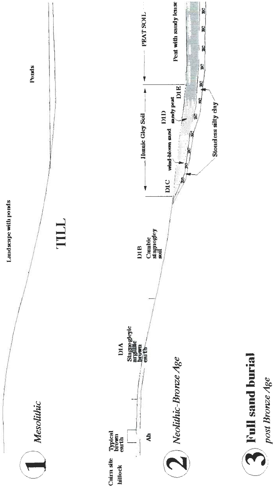
Figure 2. Tentative stages of landscape evolution around the cairn site (vertical scale exaggerated).
