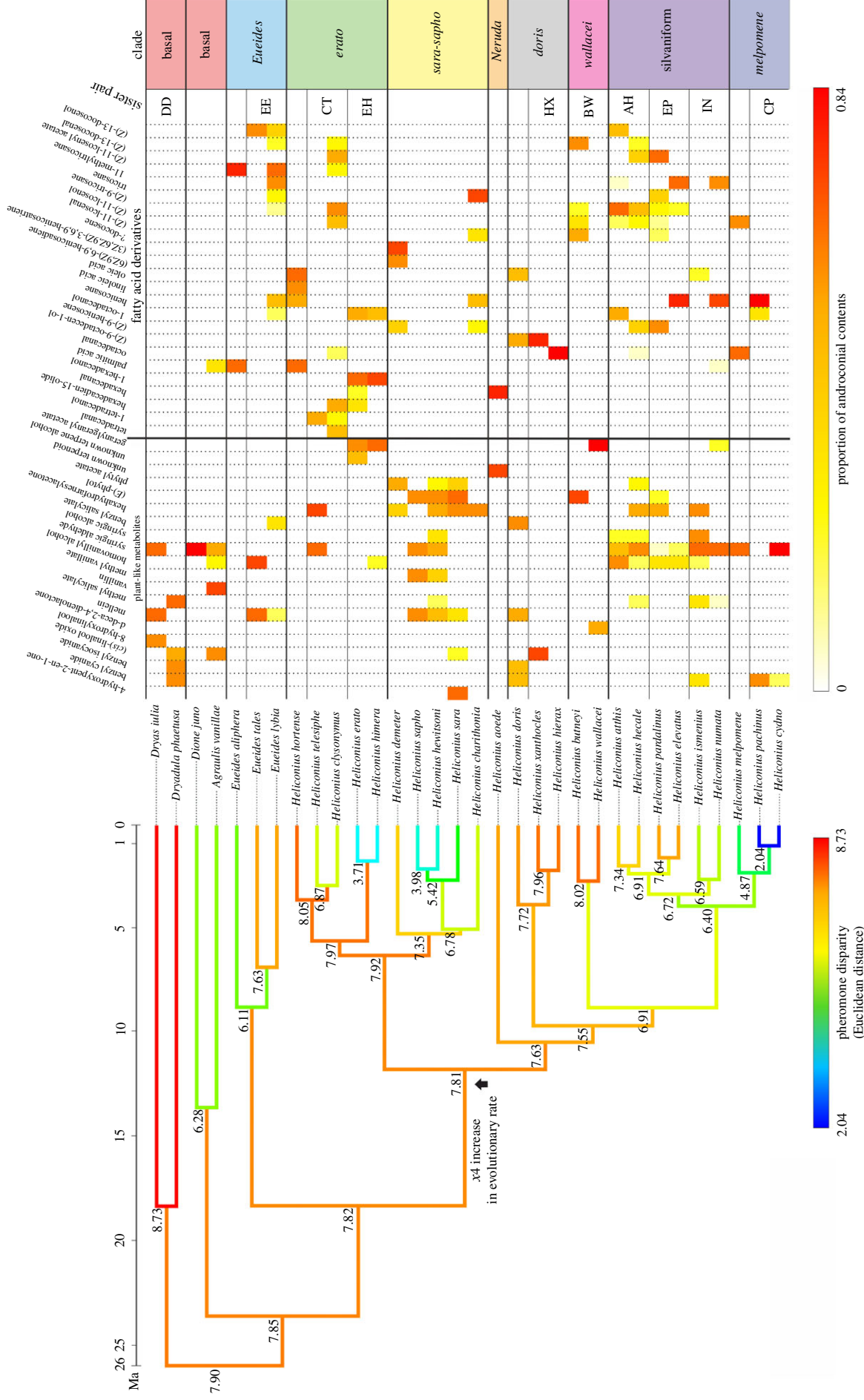
Figure 1. Heliconiini tree with branches coloured according to disparity in pheromone profiles. Values for disparity (expressed by Euclidean distance) are shown at each node. The table shows putative MSPs composition (Dataset C) of each species, where columns represent androconia-exclusive compounds and amounts are expressed as the proportion of the total androconial contents. Note the near absence Eueides and Heliconius species produce a varied cocktail comprising both plant-like metabolites and FA derivatives. This figure summarizes the most abundant compounds (at least 12% of the total androconial contents). For a complete dataset with all compounds, see (electronic supplementary material, table S6). (Online version in colour.)
