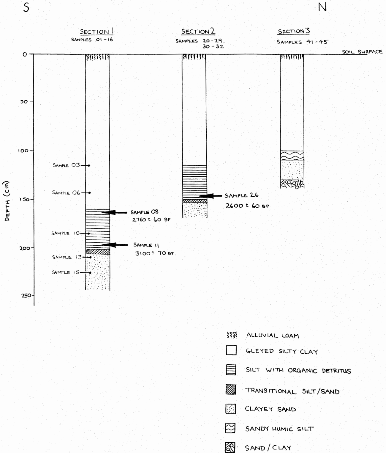
Figure 2. Stratigraphy of the North Duffield site
